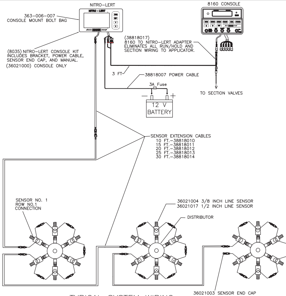
TYPICAL SYSTEM WIRING NITRO-LERT TO 8160 ADAPTER
